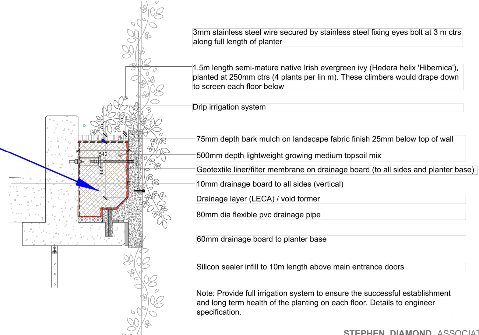
CONSTRUCTION SECTION CS-02 - SECTION THROUGH WIDER PLANTERS ZOOM IN/ Scale 1:25
