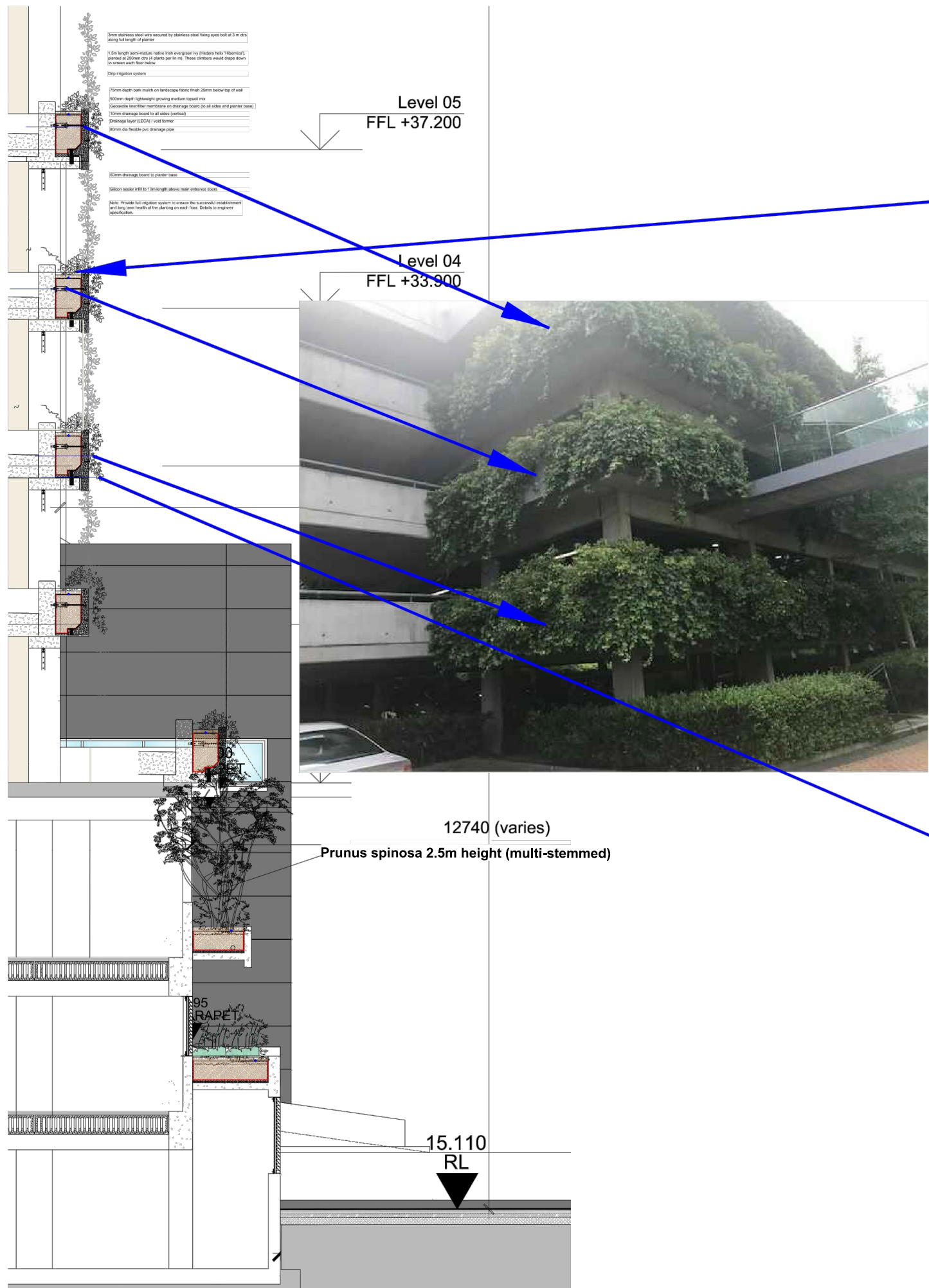
CONSTRUCTION SECTION CS-02 - SECTION THROUGH WIDER PLANTERS & ROOF GARDEN / Scale 1:100
